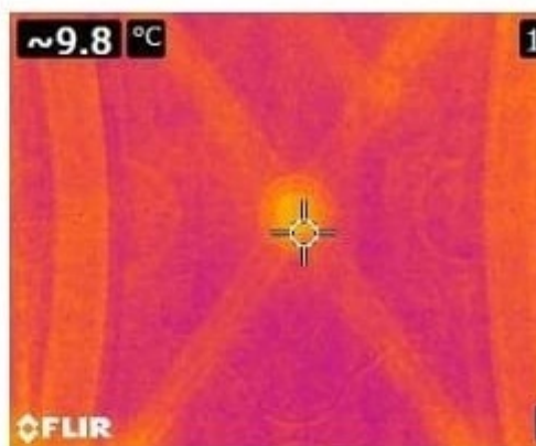
Figure 13. Thermovision picture of the arch
